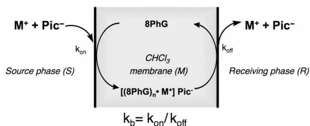
Figure 3. Representation of a symport gradient pumping mechanism. M^+ represents metal and Pic^- represents picrate. K_b is the binding constant, K_{on} is the association constant and K_{off} is the disassociation constant (adapted from reference 21).
