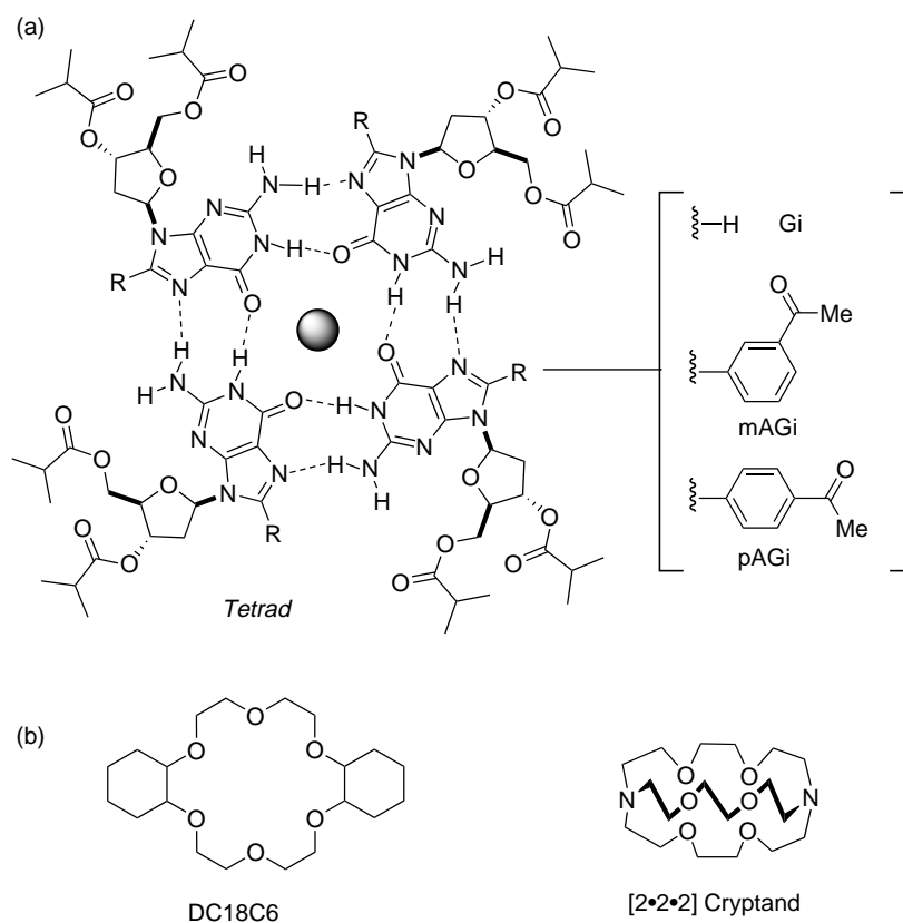
Figure 2. (a) Tetrads formed by the various 2'-deoxyguanosine derivatives shown and (b) covalent ionophores used as reference compounds.
