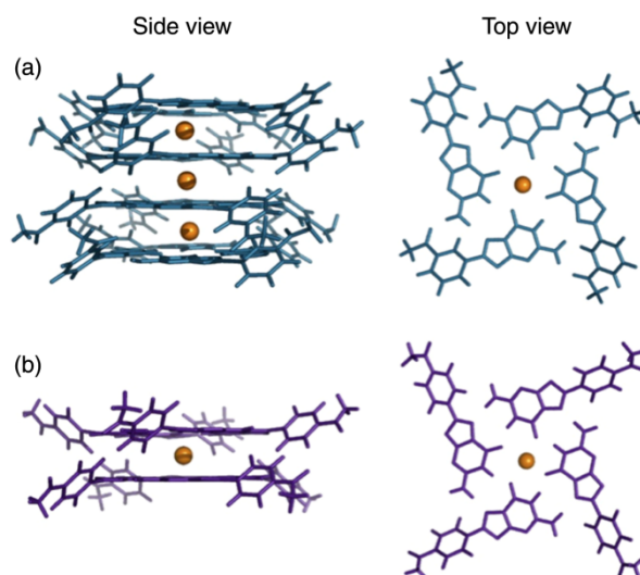
Figure 1. Side (left) and top (right) views for molecular models of (a) ( mAGi ) 16 ·3K + and (b) ( pAGi ) 8 ·K + GQs. The 2'-deoxyribose moiety and the lipophilic groups attached to it are not shown for clarity.
