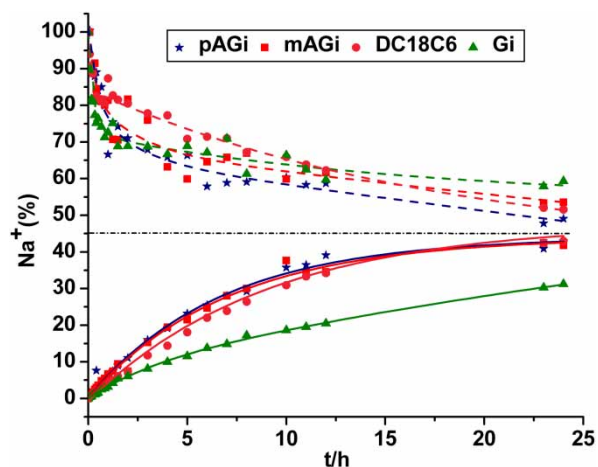
Figure 5. Extraction and transport efficiency (mol %) of sodium picrate by 8PhGs and DC18C6 for a period of 24 h at 303 K.
