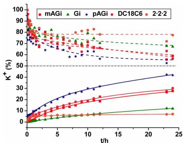
Figure 4. Extraction and transport efficiency (mol%) of potassium picrate by 8PhGs, DC18C6 and 2·2·2 for a period of 24 h at 303 K. In this and Figures 5–7, values over 50% correspond to ions moving from the source phase to the bulk membrane and those below 50% represent ions moving from the bulk membrane into the receiving phase.
