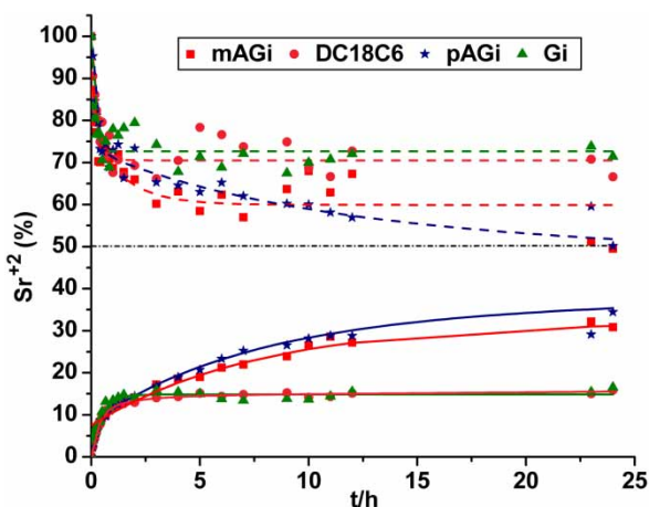
Figure 7. Extraction and transport efficiency (mol %) of strontium picrate by 8PhGs and DC18C6 for a period of 24 h at 303 K.
